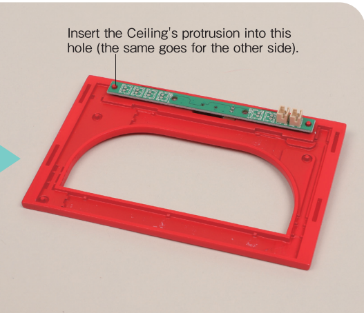
Assemble the ②Circuit Board to the ①Ceiling by fitting its terminals into the holes of the Ceiling and inserting the Ceiling's protrusions into the holes on the left and right.
