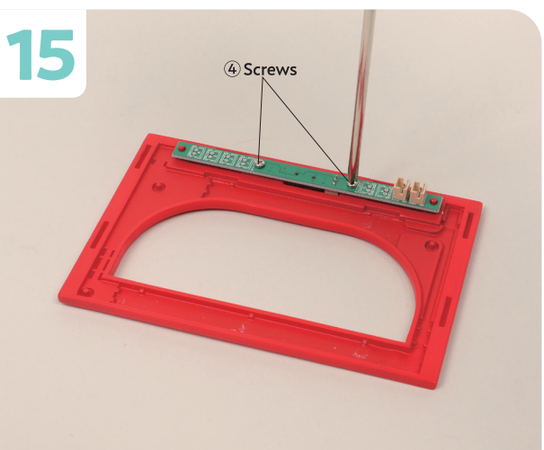
Tighten the ④Screws one by one into the two holes on the ②Circuit Board to secure it in place.
