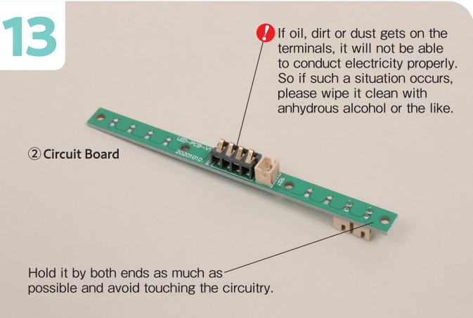
Try to hold the ②Circuit Board by both ends as much as possible and avoid touching the circuitry. Also, be very careful not to touch the terminals in the middle, as oil on your hands, dust and dirt can get on them and prevent the electricity from conducting properly.
