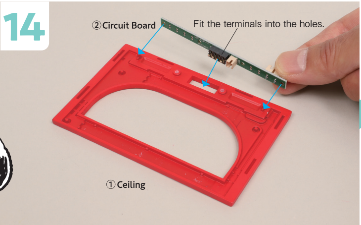
Assemble the ②Circuit Board to the ①Ceiling by fitting its terminals into the holes of the Ceiling and inserting the Ceiling's protrusions into the holes on the left and right.
