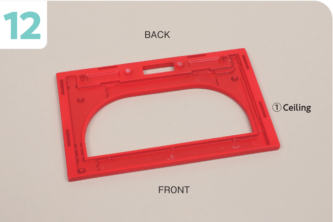
Check the orientation of the ①Ceiling—the uneven side with protrusions and holes will be the inner side that connects the Circuit Board after assembly.
